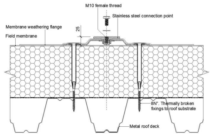
AXTER IFP-250 ON WARM ROOF – SECTION VIEW (STEEL DECK)
