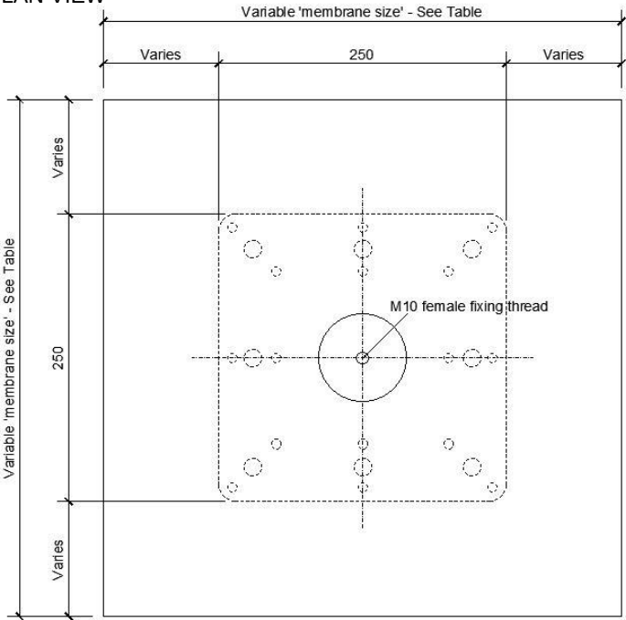
AXTER IFP-250 – PLAN INCLUDING MEMBRANE
