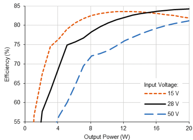
4.1.4 SVLHF2815S Efficiency (Typical, 25 °C)
