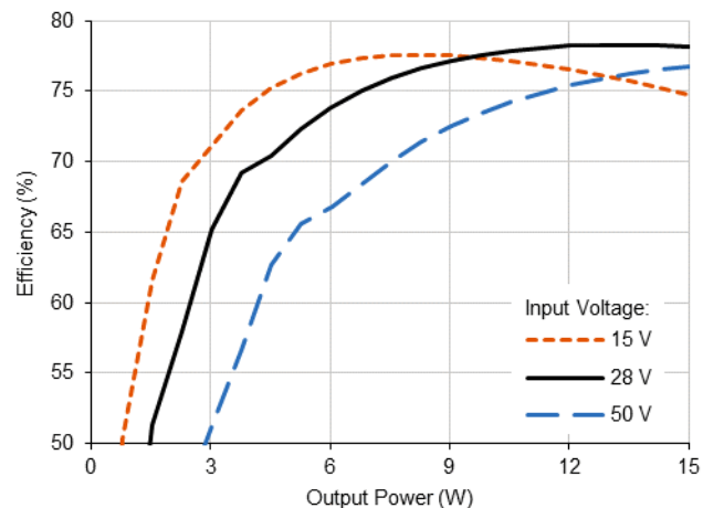
4.1.2 SVLHF2805S Efficiency (Typical, 25 °C)
