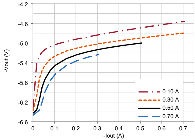
4.1.2 SVLSA5005D Cross-Regulation (Typical, 25 °C)
