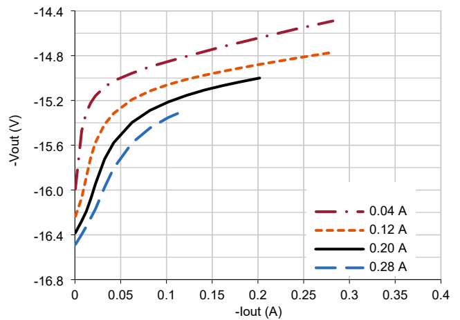
4.4.2 SVLSA5015D Cross-Regulation (Typical, 25 °C)
