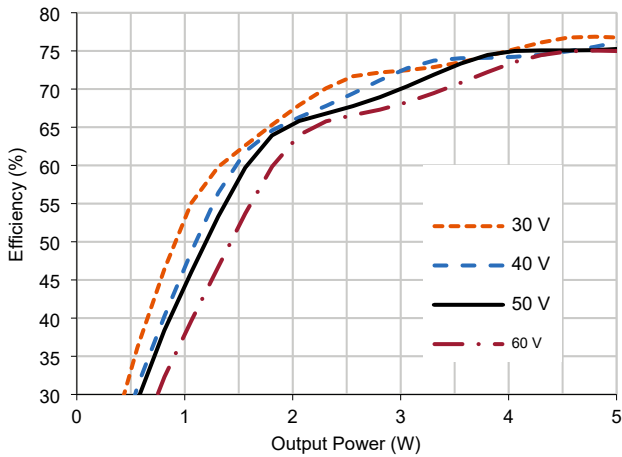
4.2.1 SVLSA5007D Efficiency (Typical, 25 °C)
