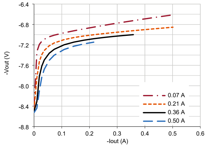
4.2.2 SVLSA5007D Cross-Regulation (Typical, 25 °C)
