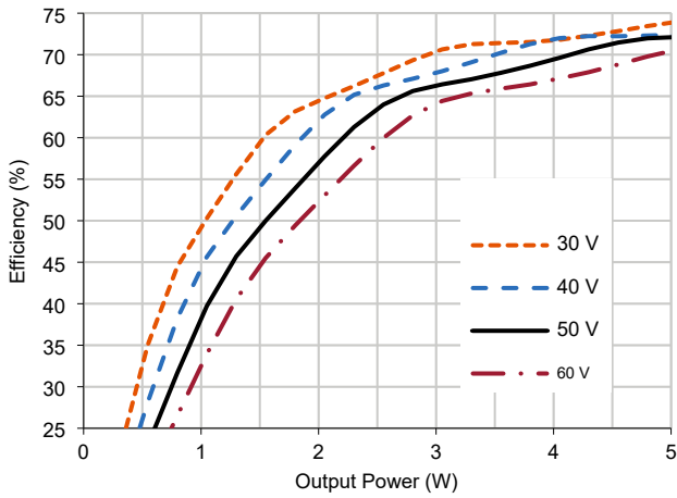
4.1.1 SVLSA5005D Efficiency (Typical, 25 °C)
