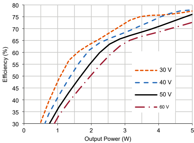
4.4.1 SVLSA5015D Efficiency (Typical, 25 °C)
