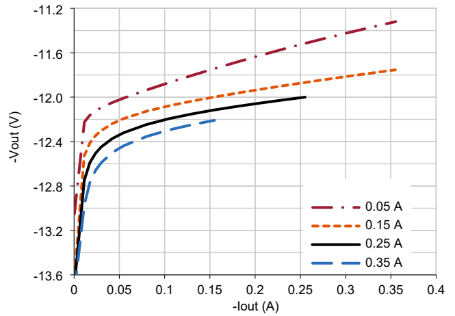
4.3.2 SVLSA5012D Cross-Regulation (Typical, 25 °C)
