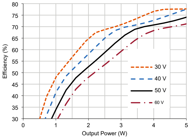
4.3.1 SVLSA5012D Efficiency (Typical, 25 °C)
