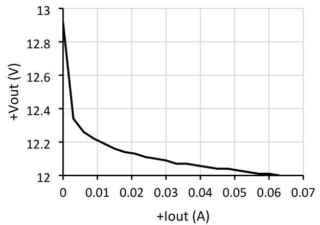
4.3.2 SVRCH2812D +Vout Load Regulation 1 (Typical, 25 °C)
