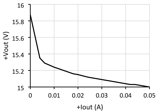
4.3.3 SVRCH2815D +Vout Load Regulation 1 (Typical, 25 °C)
