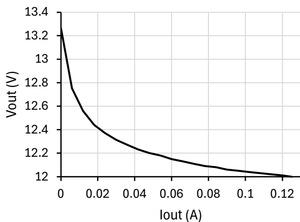
4.1.3 SVRCH2812S Load Regulation (Typical, 25 °C)
