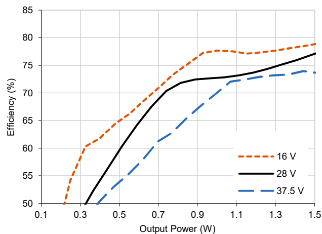
4.1.4 SVRCH2815S Efficiency (Typical, 25 °C)
