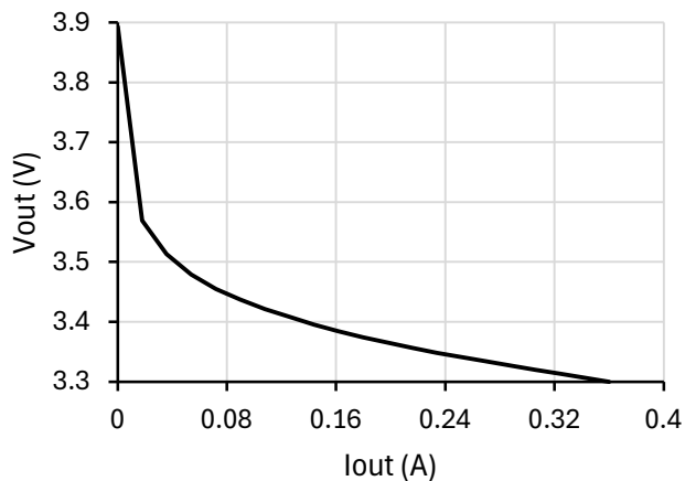
4.1.1 SVRCH283R3S Load Regulation (Typical, 25 °C)
