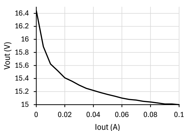
4.1.4 SVRCH2815S Load Regulation (Typical, 25 °C)
