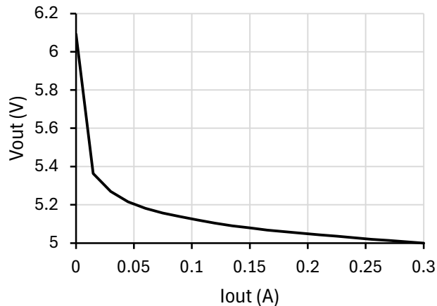
4.1.2 SVRCH2805S Load Regulation (Typical, 25 °C)
