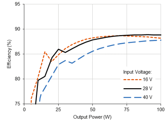
4.1.6 VPT100+2828S Efficiency (%) vs. Output Power (W)
