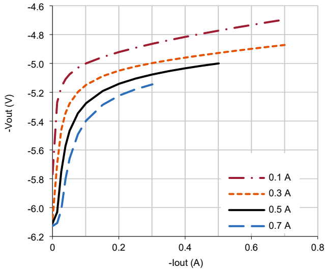
Figure 9 – VPT5-2805D -Vout (V) vs. -Iout (A)
