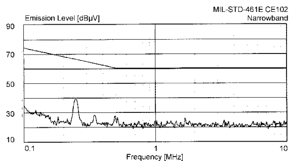
Figure 12 – MIL-STD-461D/E Two VPT30-2800S and One VPT100-2800S With VPTi10-28 Input Module
