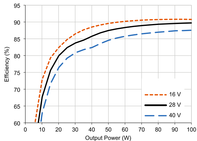
4.1.4 VSC100-2815S Efficiency (Typical, 25 °C)
