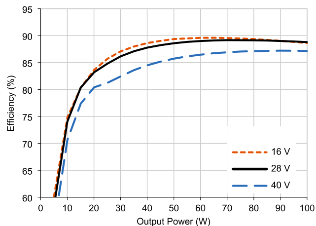
4.1.2 VSC100-2805S Efficiency (Typical, 25 °C)
