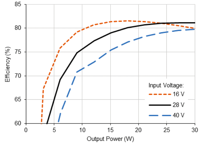
4.1.2 VSC30-2805S Efficiency (Typical, 25 °C)
