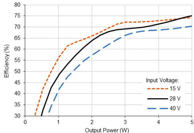
4.1.2 VSC5-2805S Efficiency (Typical, 25 °C)
