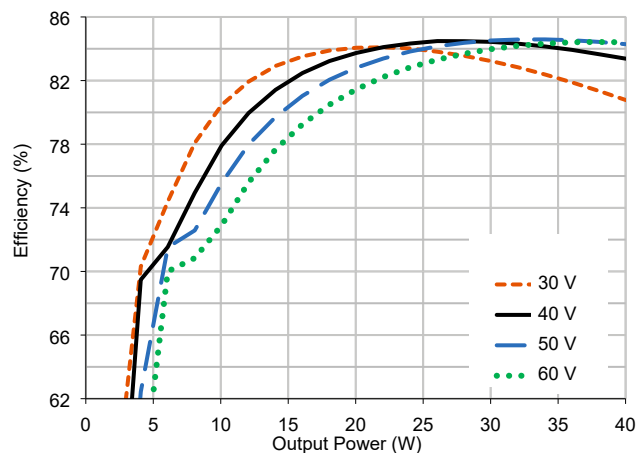
4.1.3 SVLTR5012S Efficiency (Typical, 25 °C)
