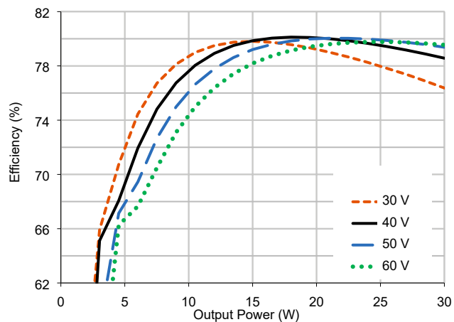
4.1.2 SVLTR5005S Efficiency (Typical, 25 °C)
