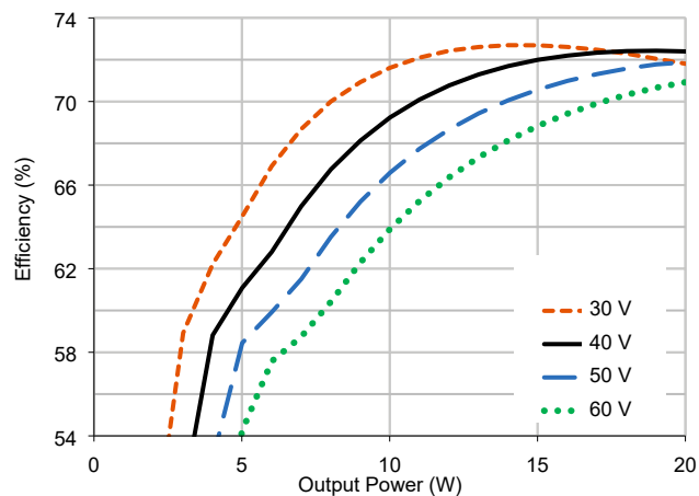
4.1.1 SVLTR503R3S Efficiency (Typical, 25 °C)
