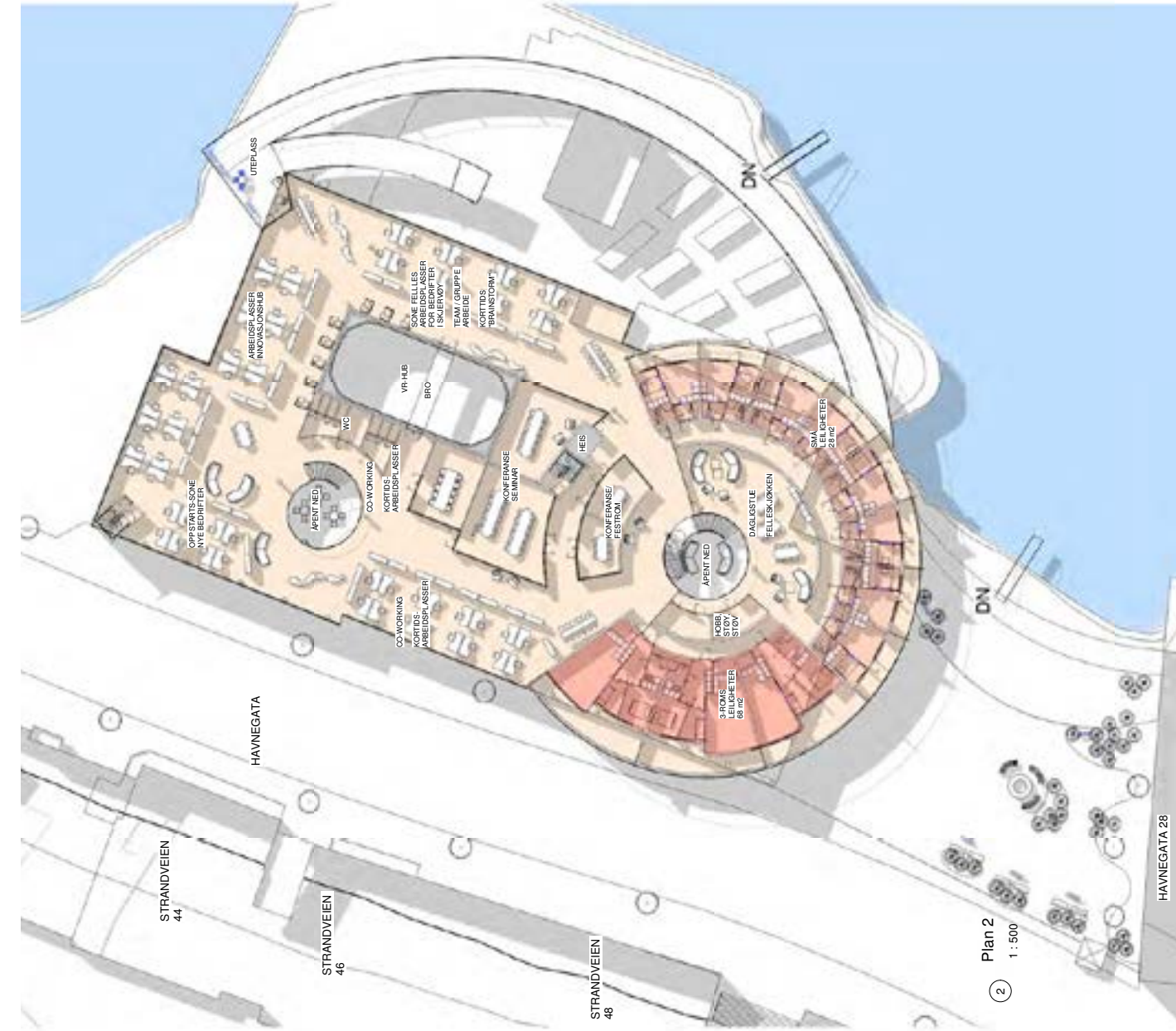
Plan 1 1:500
