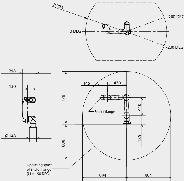
Working range CRX-5iA Food Grade
