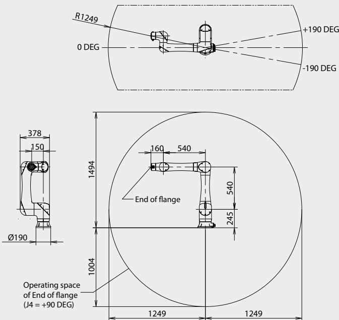
Working range CRX-10iA Food Grade
